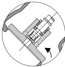
Relief plug / By-pass disk
